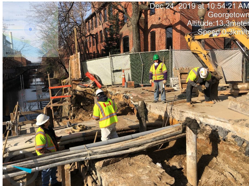
Excavation at Bridge's North Abutment
