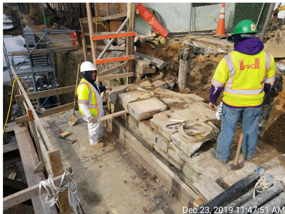
Excavation for the Bridge's North Abutment Footing
