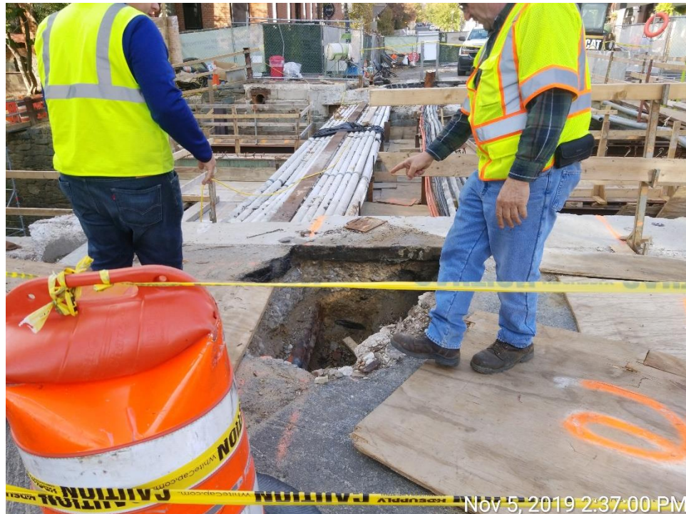
Measuring the Conflict Between Pile 3 and Verizon Manhole
